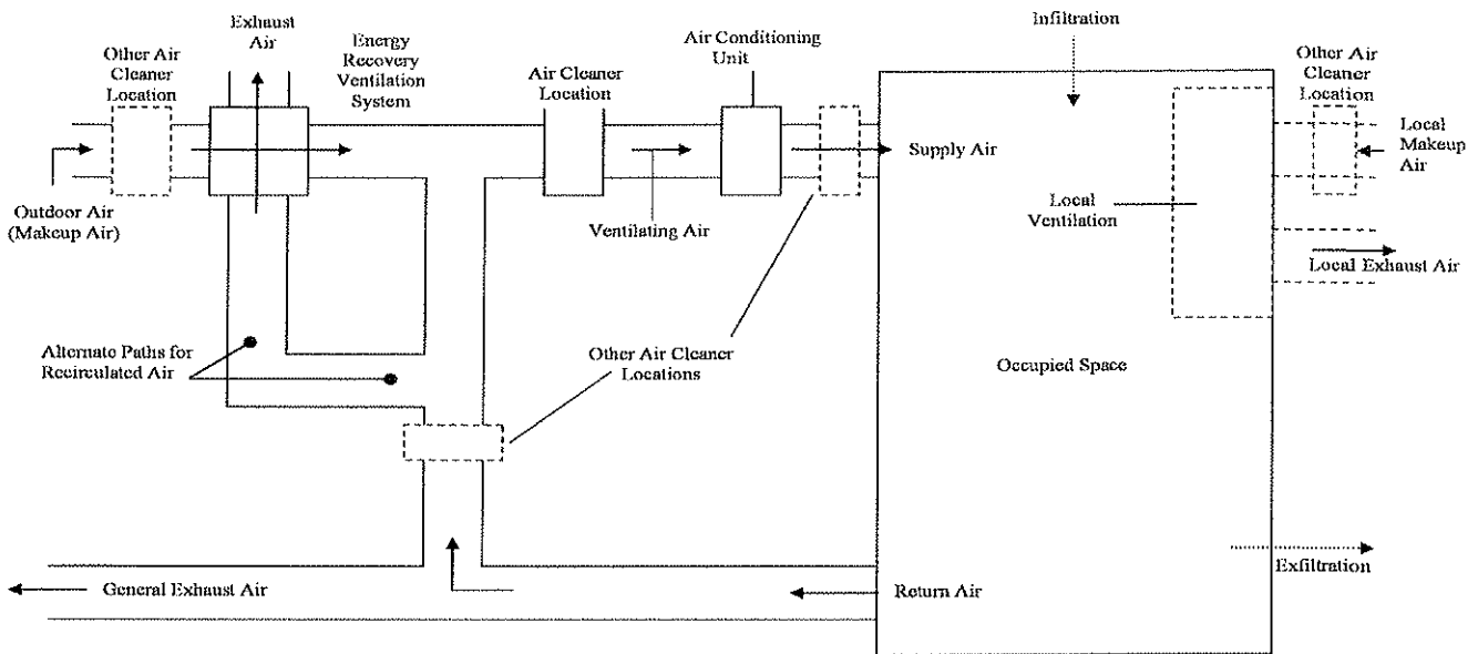
Figure 3.1 Ventilation system.
