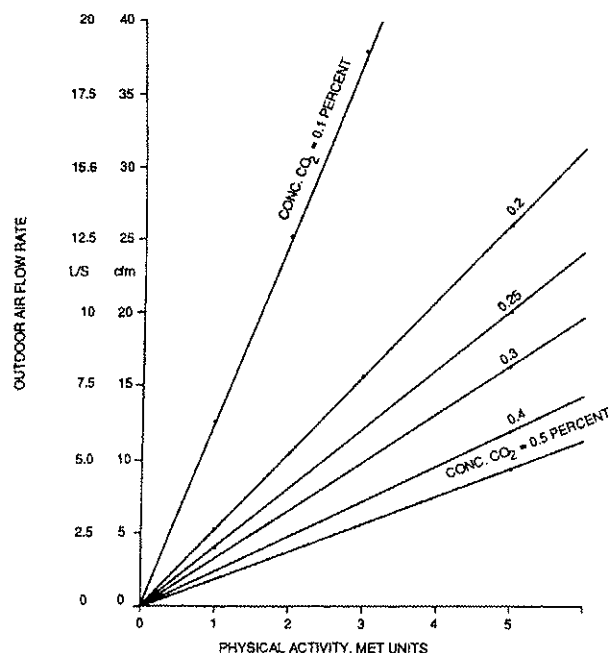
Figure C-3 Ventilation requirements.
