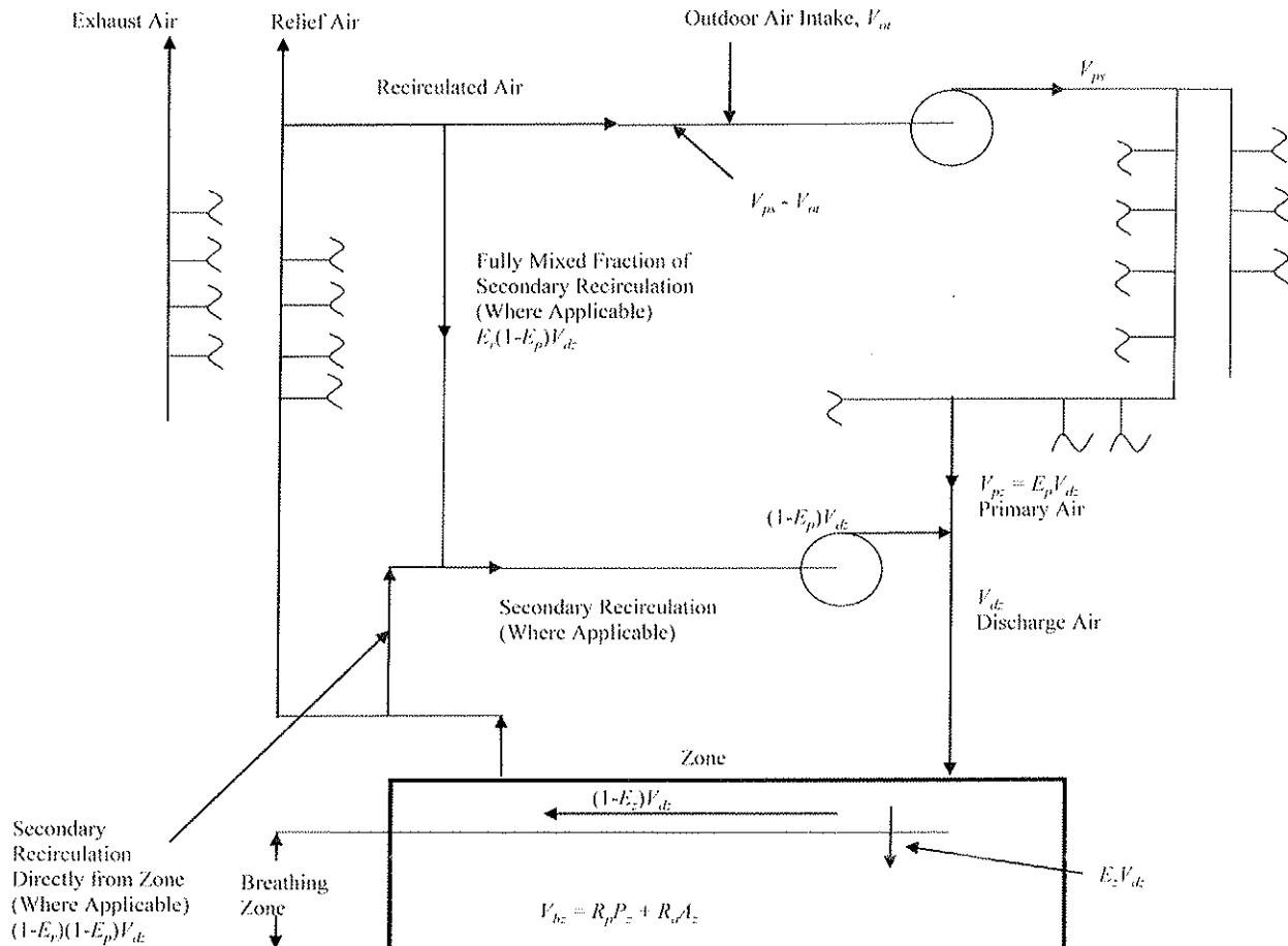
FIGURE A-1 Ventilation system schematic.
